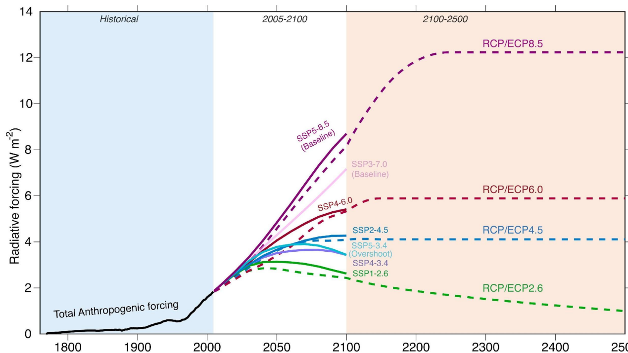
Figure SM1.1: Radiative forcing ( W m^{-2} ) time series for historical data (1765–2004), and for future scenarios from the Representative Concentration Pathways (RCP; 2005–2100) and their continuation as the extended RCPs (2100–2500), and the Shared Socio-economic Pathways (SSP; 2005–2100). The RCP scenarios are shown as dashed curves, and SSPs are shown as solid curves ('Marker' scenarios are used). Note the change in x-axis scale for the 2005–2100 interval to give an improved illustration of radiative forcing scenarios during the 21st century.
