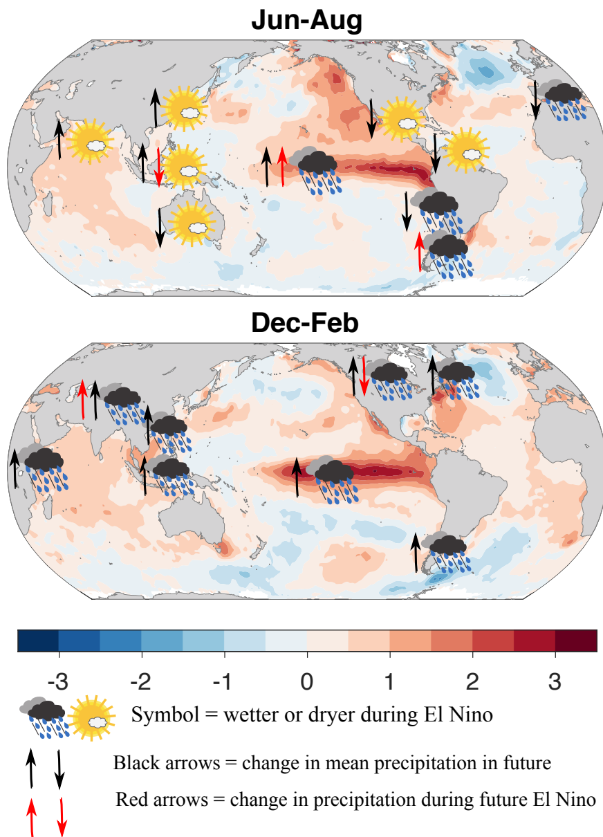
Figure 6.6: Schematic figure indicating future changes in El Niño teleconnections based on the study of Power and Delage (2018). The background pattern of sea surface temperature anomalies ( ^{\circ}\text{C} ) are averaged from June 2015 to August 2015 (panel a) and December 2015 to February 2016 (panel b), during the most recent extreme El Niño event (anomalies computed w.r.t. 1986–2005). Symbols indicate present-day teleconnections for El Niño events. Black arrows indicate if there is a model consensus on change in mean rainfall in the region. Red arrows indicate if there is a model consensus on change in the rainfall anomaly under a future El Niño event. Direction of the arrow indicates whether the response in precipitation is increasing (up) or decreasing (down). Significance is determined when two-thirds or more of the models agree on the sign.
