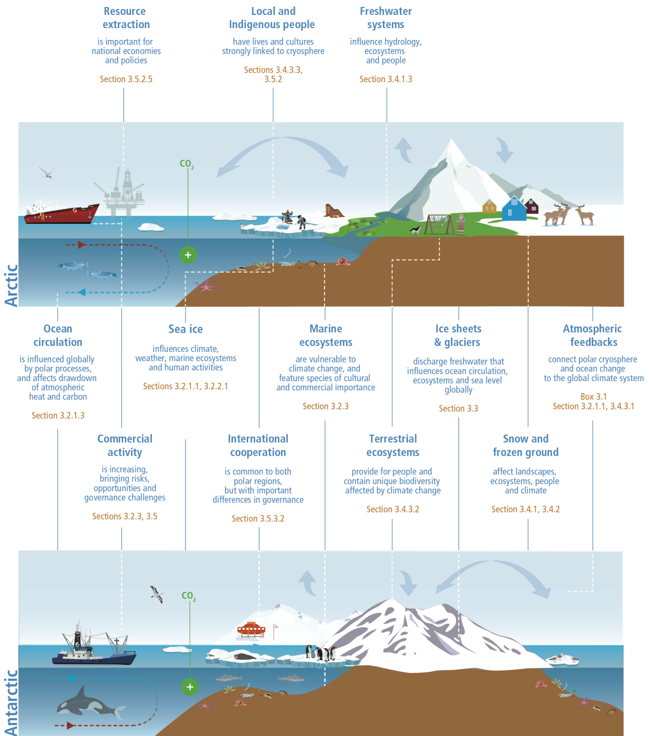
Figure 3.1: Schematic of some of the key features and mechanisms assessed in this Chapter, and by which the cryosphere and ocean in the polar regions influence climate, ecological and social systems in the regions and across the globe. Specific elements are labelled, and section numbers given for where detailed assessment information can be found.
