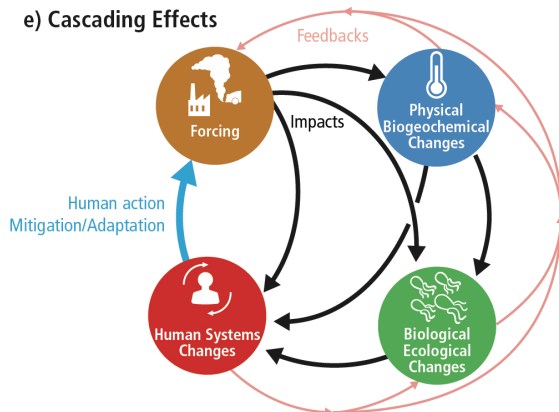
Figure 1.1: Schematic of key concepts associated with changes in the ocean and cryosphere. (a) Differing responses of systems to gradual forcing (e.g., linear, delayed, abrupt, non-linear). (b) Evolution of a dynamical system in time,
