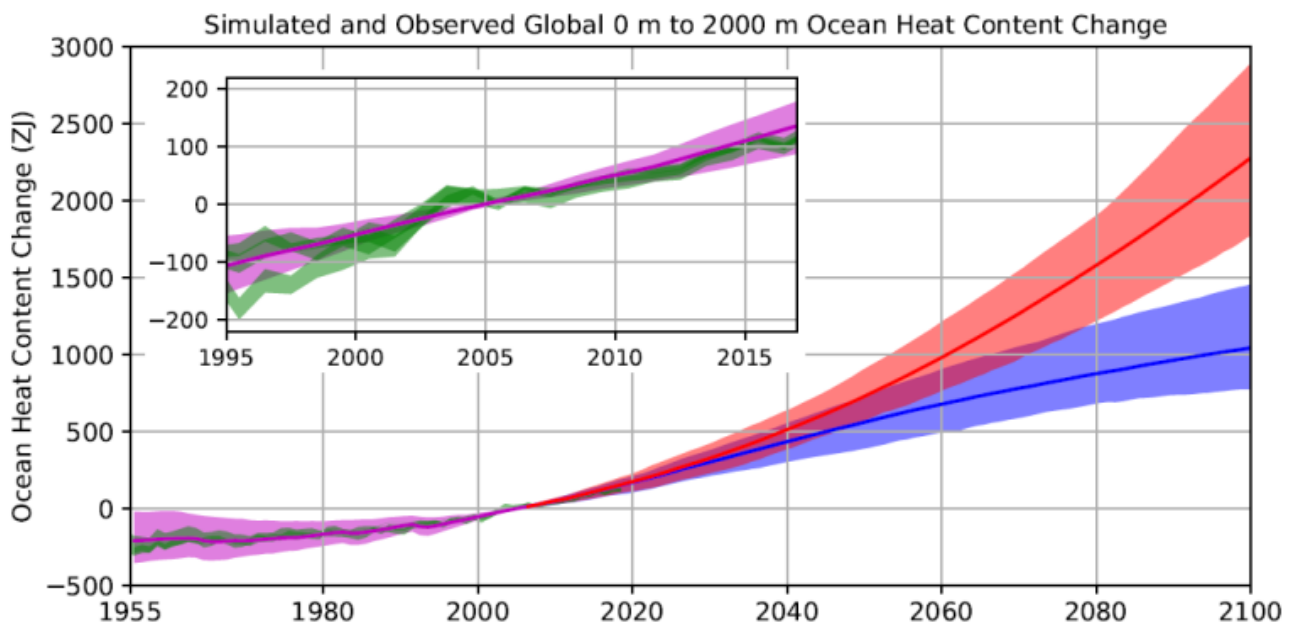
Figure 5.1: Time series of globally integrated upper 2000 m ocean heat content changes in ZJ, relative to the 2000 to 2010 period average, as inferred from observations (green) and as simulated for historical (magenta), RCP2.6 (blue) and RCP8.5 (red) forcing by a 25-member ensemble of CMIP5 ESMs ((Cheng et al., 2019). The shaded green in the outer panel is the very likely range determined by combining data from 4 long-term estimates (Green lines; Palmer et al., 2007; Levitus et al., 2012; Lyman and Johnson, 2014; Cheng and Chen, 2017; Cheng et al., 2017; Ishii et al., 2017) processed as in Johnson et al. (2018). The magenta, blue and red lines are the ESM ensemble means, while shading shows each ensemble's 5 th to 95 th percentile range. In the inset subpanel, the 4 different shaded green areas are the reported very likely range of heat content changes as inferred from observations by 4 independent groups (Green lines; Palmer et al., 2007; Lyman and Johnson, 2014; Cheng and Chen, 2017; Cheng et al., 2017; Ishii et al., 2017) processed as in Johnson et al. (2018). In the inset subpanel the RCP2.6 and RCP8.5 projections after 2005 are combined into a single ensemble with the historical simulations.
